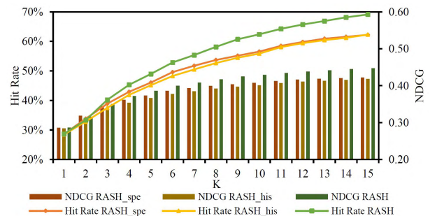
FIGURE 7. Hit rate and NDCG for RASH and its variants.
