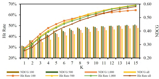
FIGURE 6. Hit rate and NDCG for different number of candidate APIs.
