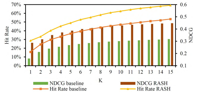
FIGURE 14. Hit rate and NDCG for different approaches.
