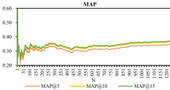
FIGURE 12. MAP for different number of questions.
