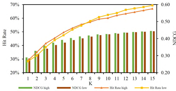
FIGURE 9. Hit rate and NDCG for different subsets.
