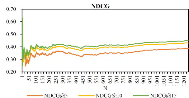
FIGURE 11. NDCG for different number of questions.
