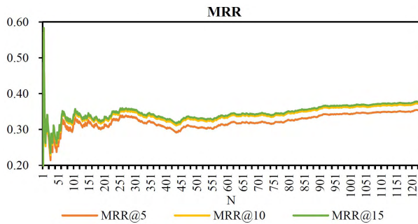
FIGURE 13. MRR for different number of questions.
